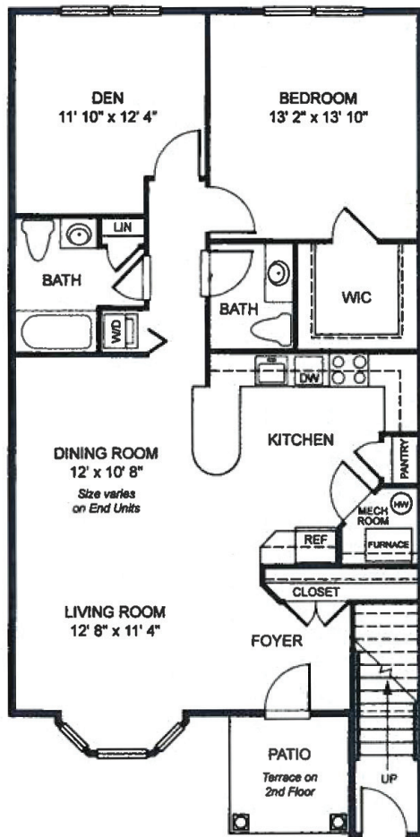
One bedroom 1st floor – 1,148 sq ft
